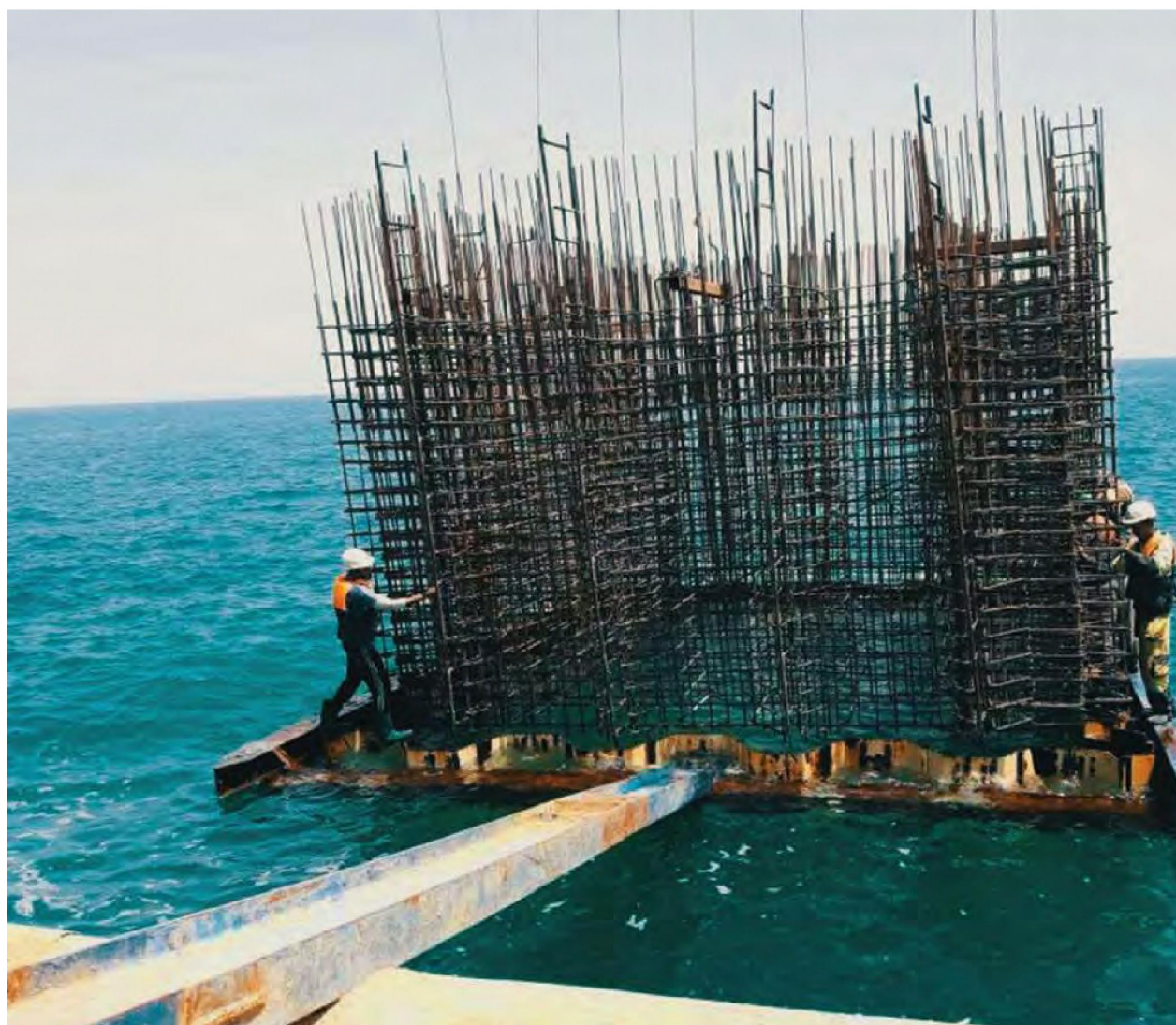
Development of EHC - OPC gas tankers berth
